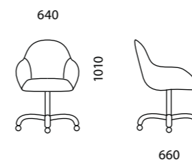
D80 640x660x1010
